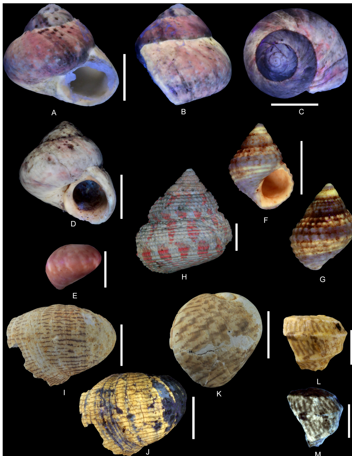
Fig 5. Residual colour patterns in Vetigastropoda and Neritimorpha. (A–G, I–K) Gastropods from the Oxfordian of Cordebugle (Calvados). (A, B) Ataphrus ( Ataphrus ) marschmidti Gründel and Kaim, 2006, MNHN.F.J11070 (Cossmann coll.). (A) apertural view. (B) labral view. (C) A. (A.) marschmidti , MNHN.F.J11074 (Cossmann coll.), apical view. (D) A. (A.) marschmidti , UPMC-136 (Le Marchand coll.), apertural view. (E) A. (Endianaulax) sarahae (Chavan, 1954), UPMC-137 (Le Marchand coll.), dorsal view. (F, G) Gerasimovcyclus cf. lorioli (Schmidt, 1905), MNHN.F.J10402 (Cossmann coll.). (F) apertural view. (G) dorsal view. (H) Calliophthalmus ( Calliophthalmus ) squamulosus (Lamarck, 1804) from the Lutetian of the Paris Basin showing red fluorescence, MNHN.F.A24999 (Pacaud coll.), dorsal view. (I, J) Neridomus ovula (Buvignier, 1843), MNHN.F.A32286 (de Morgan coll.), dorso-labral view.
