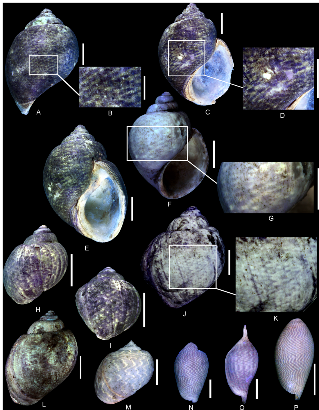
Fig 10. Residual colour pattern of Ampullina clio (d'Orbigny, 1850) from the Oxfordian of Cordebugle (Calvados). (A-L) Ampullina clio . (A-E) MNHN. F.J10210 (Cossmann coll.). (A) ablabral view. (B) detailed view of the colour pattern. (C) apertural view. (D) detailed view of the colour pattern. (E) aperturo-labral view. (F, G) MNHN.F.J10426 (Cossmann coll.). (F) apertural view. (G) detailed view of the colour pattern. (H, I) MNHN.F.J10425 (Cossmann coll.). (H) dorsal view. (I) labro-dorsal view. (J, K) MNHN.F.A46211 (Bigot coll.). (J) dorsal view. (K) detailed view of the colour pattern. (L) MNHN.F.A30347 (de Morgan coll.), dorsal view. (M-P) Gastropods from the Eocene of the Paris basin showing a similar meshwork pattern. (M) Globularia (Globularia) patuloides (Cossmann and Pissarro, 1902), MNHN.F.A31162 (Faullummel coll., Bartonian), dorsal view. (N) Diameza (Miniseraphs) eratoides (Cossmann, 1889), MNHN.F.A28934 (Pacaud coll., Lutetian), dorsal view. (O) D. (Diameza) fragilis (Defrance, 1825), MNHN.F.A28939 (Pacaud coll., Lutetian), dorsal view. (P) D. (Miniseraphs) isabella (Bernay in Deshayes, 1865), MNHN.F.A28936 (Pacaud coll., Lutetian), dorsal view. Scale bars: 10 mm (A, C, D, E, H-J, M), 5 mm (B, F, G, K, O), 2 mm (M, N).
