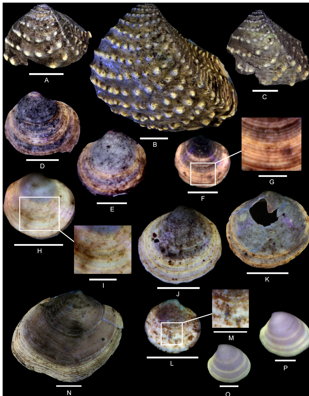
Fig 13. Residual colour patterns of bivalve species (Trigonioida and Lucinoidea) from the Oxfordian of Cordebugle (Calvados). (A-M) Bivalves from the Oxfordian of Calvados (Cordebugle). (A) Myophorella nodulosa (Lamarck, 1801), UPMC-139 (UPMC coll.), left valve view. (B) M. nodulosa , UPMC-138 (UPMC coll.), left valve view. (C) M. nodulosa , UPMC-140 (UPMC coll.), left valve view. (D) Mesolinga typica Chavan, 1952, MNHN.F.J11589 (Cossmann coll.), left valve view. (E) M. typica , MNHN.F.J11590 (Cossmann coll.), right valve view. (F, G) Mesomiltha pulchra (Zittel and Goubert, 1861), UPMC-144 (Le Marchand coll.). (F) left valve view. (G) detailed view of the colour pattern. (H, I) Jagonoma circumcisa (Zittel and Goubert, 1861), MNHN.F.J11586 (Cossmann coll.). (H) right valve view. (I) detailed view of the colour pattern. (J) J. circumcisa , MNHN.F.J11588 (Cossmann coll.), left valve view. (K) J. circumcisa , MNHN.F.J11587 (Cossmann coll.), left valve view. (L, M) J. circumcisa , MNHN.F.J11585 (Cossmann coll.). (L) right valve view. (M) detailed view of the colour pattern. (N-P) Bivalves from the Lutetian of the Paris basin showing similar commarginal stripes. (N) Pseudomiltha (Pseudomiltha) mutabilis (Lamarck, 1807), MNHN.F.A25068 (Faullummel coll.), left valve view. (O, P) Katelysia (Textivenus) scobinellata (Lamarck, 1806). (O) MNHN.F.A31917 (Faullummel coll.), right valve view. (P) MNHN.F.A31910 (Faullummel coll.), right valve view. Scale bars: 10 mm (A-C, J, K, N), 5 mm (D-F, H, L, O, P), 2 mm (G, I, M).
