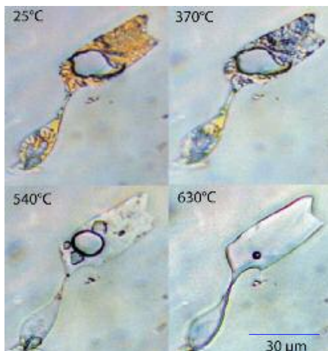
Facing page: A thin film on a partly healed cleavage in topaz, 30X Tepetate, San Luis Potosí, Mexico; John Koivula photo
