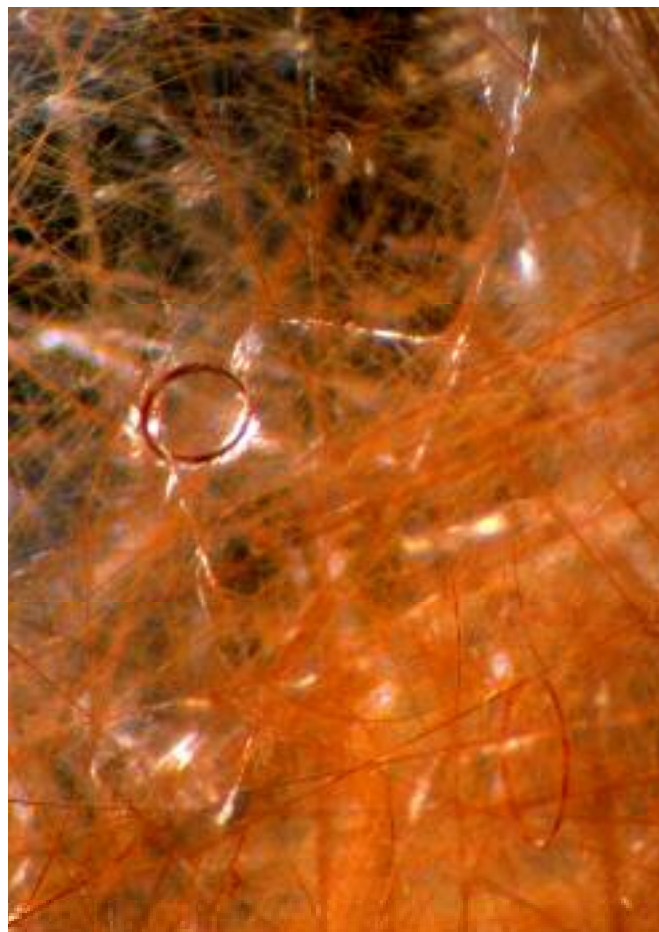
Above: Topaz with goethite alteration rings and etched dislocation channels (10x)
