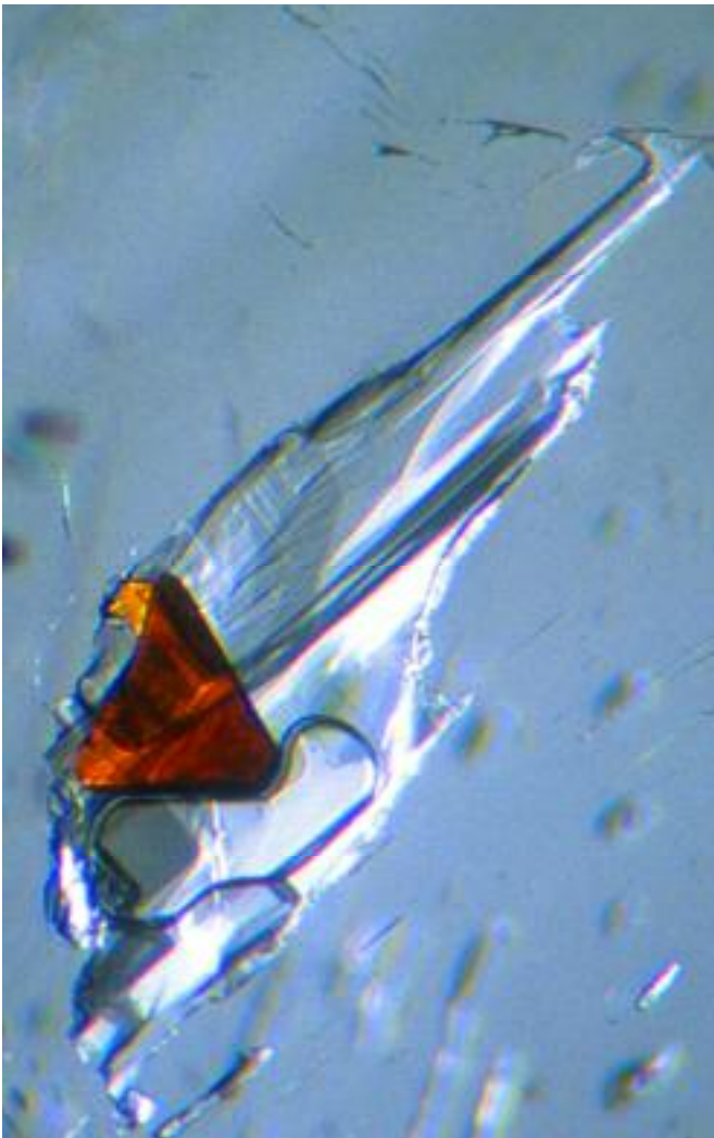
Above: Spessartine (5.07 mm long) inclusion in topaz from Brazil
