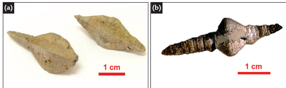
Figure 5 (a). Typical anatase crystals showing double bipyramidal forms from the Datas de Cima deposit. (b). A more elongated crystal from this deposit, showing different forms in its central part.
