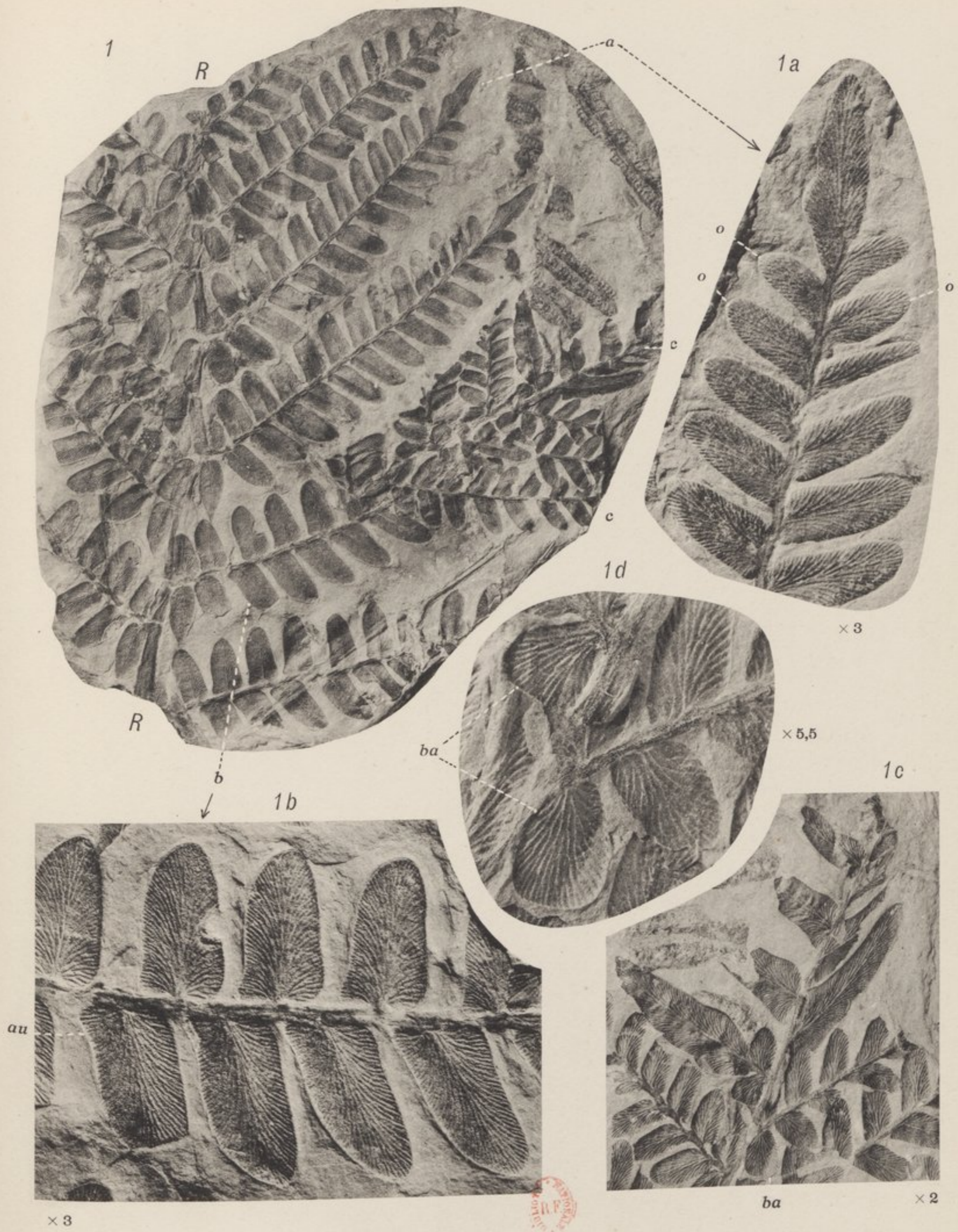
MIXONEURA DEFLINEI nov. sp.
