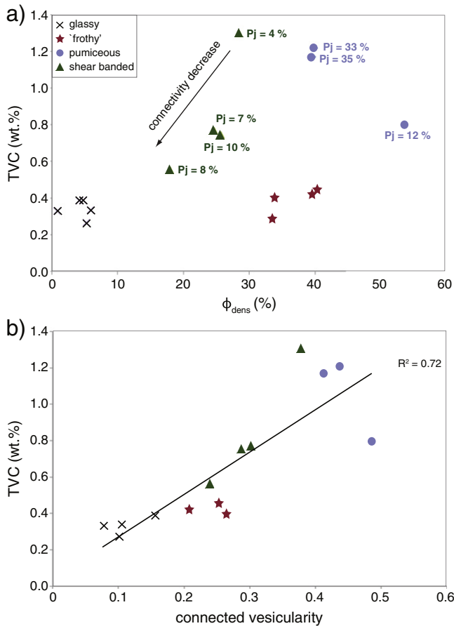
Fig. 17. a) Total volatile content TVC [wt.%] against total vesicularity [%] and b) TVC [wt.%] against connected vesicularity. P_j values for pumiceous and shear banded samples are indicated. Arrow shows decrease in connected vesicularity of shear banded samples with decreasing vesicularity, also shown in b).
