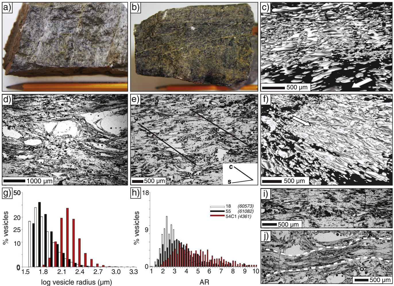
Fig. 6. Representative images of shear banded RR samples. a) and b) Photographs of samples 54C1 and 54C2 showing sheared vesicle textures and obsidian bands. c) 3D rendered image of sample 55 illustrating high vesicle connectivity and irregular vesicle shapes. d) and e) Optical microscope images of samples 54C1 and 55, respectively, showing sigmoidal, high AR sheared vesicles, shear banding and S–C fabric in e). Inset shows orientation of S and C planes. f) 3D rendered image of sample 54C1 illustrating very high vesicle connectivity, elongation parallel to shear and localised differences in vesicle content. Arrows show sense of local shear. g) Vesicle size distribution VSD and h) aspect ratio AR histograms of type 4 lavas analysed in 3D. Vertical axis on both plots is number of vesicles as a percentage of total vesicles in the sample. Horizontal axis on VSD plot is the logarithm of the equivalent spherical vesicle radius. Italic figures in brackets show number of vesicles analysed per sample. i) and j) Optical microscope images showing a plane of connected vesicular pore space parallel to shear in sample 54C1 and shear banding in sample 18, respectively.
