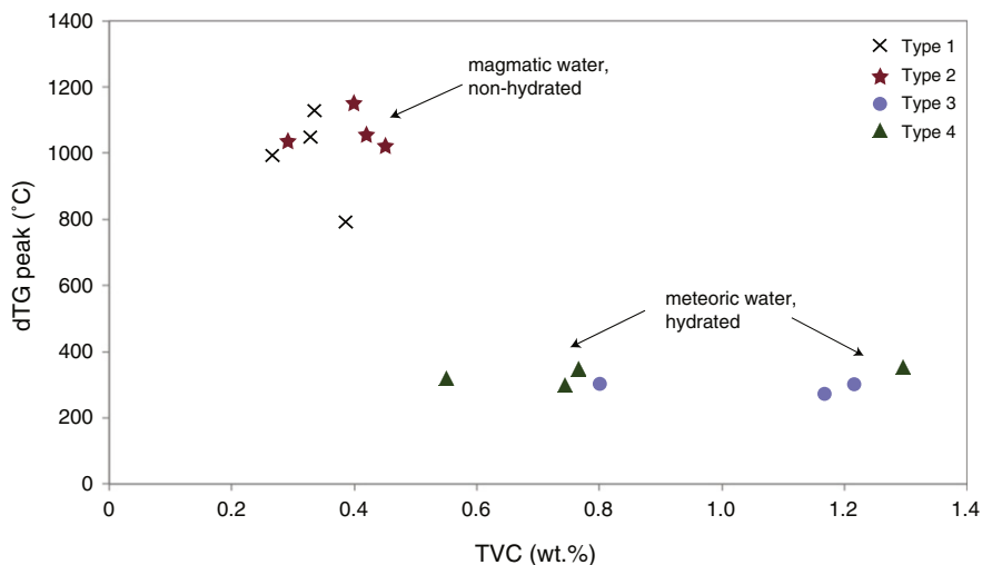
Fig. 16. Peak degassing temperature of RR samples against total volatile content TVC. Symbols show RR lava types, described in Section 3.1.
