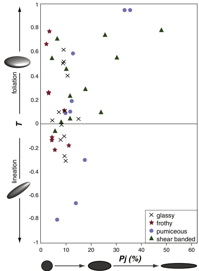
Fig. 15. Plot of AMS shape parameter T against degree of anisotropy P_j . T > 0 = oblate fabrics T < 0 = prolate fabrics. Increasing P_j indicates increasing shear strain.
