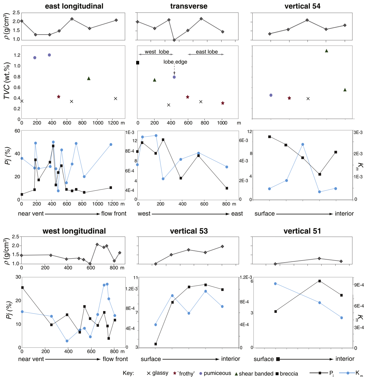
Fig. 12. Longitudinal, transverse and vertical transects of several properties of the RR lava flow. Transects show variation in bulk density \rho , total volatile content TVC (data only obtained for east longitudinal, transverse and vertical 54 transects), bulk susceptibility K_m and degree of anisotropy P_j . All error bars are smaller than the size of the symbols. Transect locations are shown in Fig. 1. X-axis scale for vertical transects is not known but samples were taken at approximately equal intervals over vertical heights of 3–5 m.
