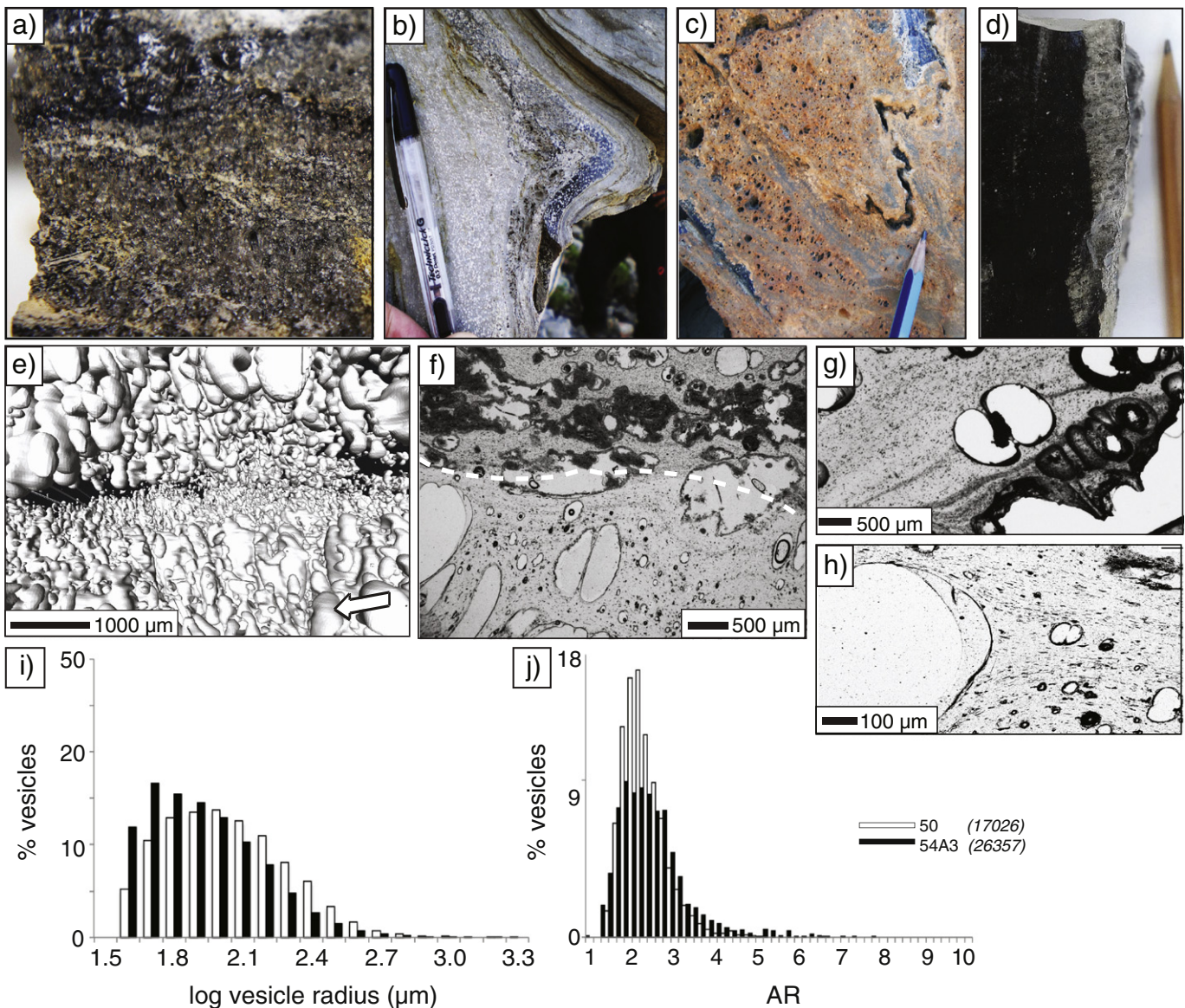
Fig. 4. Representative images of 'frothy' obsidian RR samples. a) Photograph of type 2 lava (sample 50) in an ~10 cm wide fold hinge (shown in c)) b) Localised 'frothy' lava in fold hinge of banded spherulitic obsidian. c) Micro-parasitic folds in vesicular and non-vesicular obsidian bands. d) Localised planar vesicle-rich lava in a glassy obsidian sample. e) 3D rendered image of sample 50 showing sub-spherical vesicles elongated perpendicular to shear with some coalescence parallel to shear. Sample also contains a glassy obsidian band parallel to shear shown by the absence of vesicles. Sense of local shear shown by arrows. f) Optical microscope image of sample 54A3 showing banded microlite-rich (top) and microlite-poor (bottom) layers as well as variable vesicle sizes. g) and h) Optical microscope images showing overprinting of microlite-defined flow fabric by vesicles in sample 51A1 and deflection of microlite-defined flow fabric by a vesicle in sample 54A3, respectively. i) Vesicle size distribution VSD and j) aspect ratio AR histograms of type 2 lavas analysed in 3D. Vertical axis on both plots is number of vesicles as a percentage of total vesicles in the sample. Horizontal axis on VSD plot is the logarithm of the equivalent spherical vesicle radius. Italic figures in brackets show number of vesicles analysed per sample.
