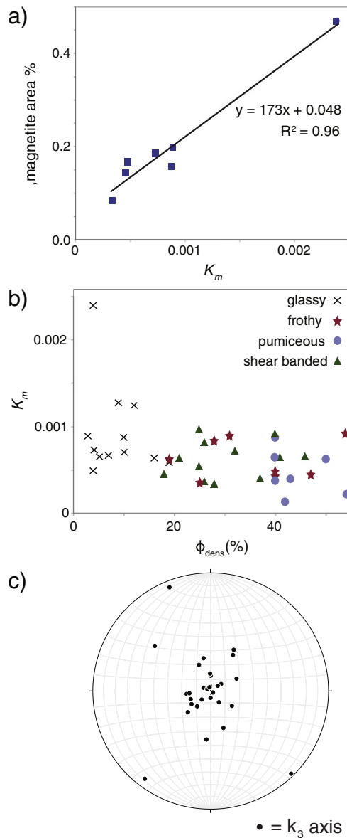
Fig. 14. a) Amount of magnetite (% of thin section area), calculated from optical microscope images of thin sections, against bulk susceptibility K_m . Solid line shows best linear fit of data. b) Bulk susceptibility K_m against vesicularity for each lava type. c) Stereographic projection of all samples with oblate AMS ellipsoids, showing a predominantly sub-vertical k_3 orientation, indicating foliations parallel to the shear plane.
