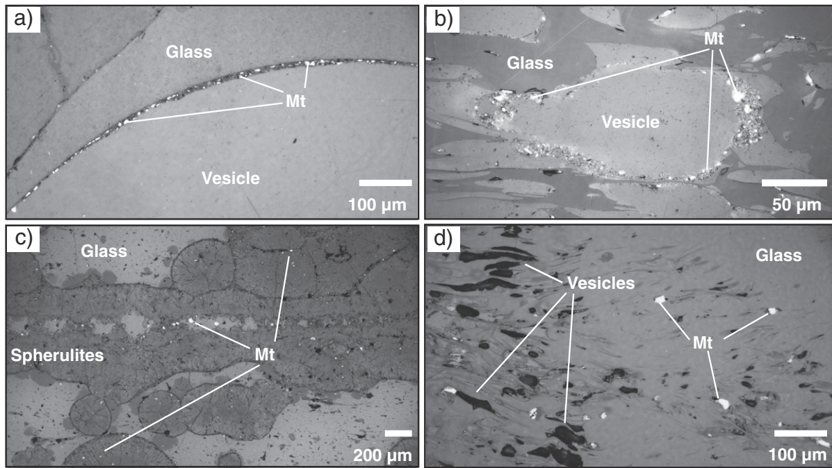
Fig. 13. Reflected light images of RR thin sections showing magnetite distributions a. and b. clustered on vesicle rims, c. within spherulite trails and d. sparse magnetite grains in the glass matrix.
