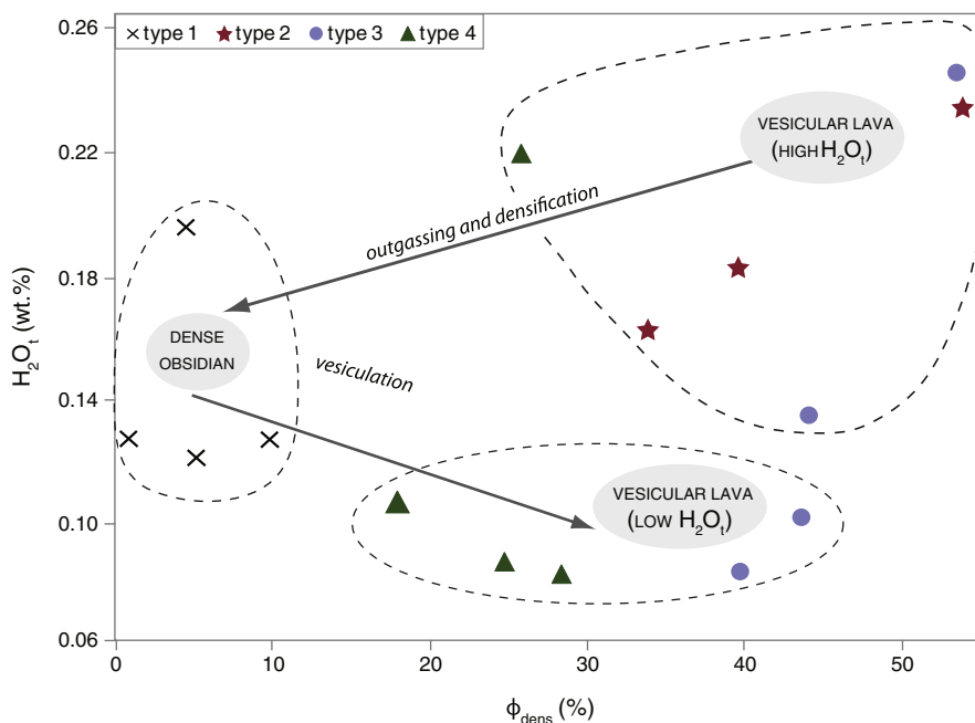
Fig. 20. Magmatic water content [wt.%] of RR samples against vesicularity [%], showing inferred outgassing and vesiculation paths between lava samples.
