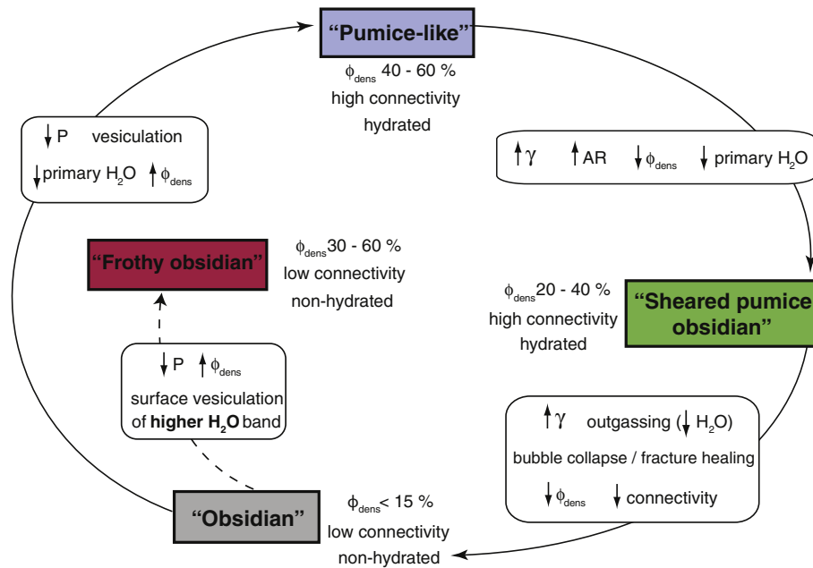
Fig. 21. Model for generation of RR lavas, with lava types representing the final stages of the shearing cycle before complete cooling. \phi_{dens} is vesicularity, \gamma is shear strain, AR is vesicle aspect ratio and P is pressure.
