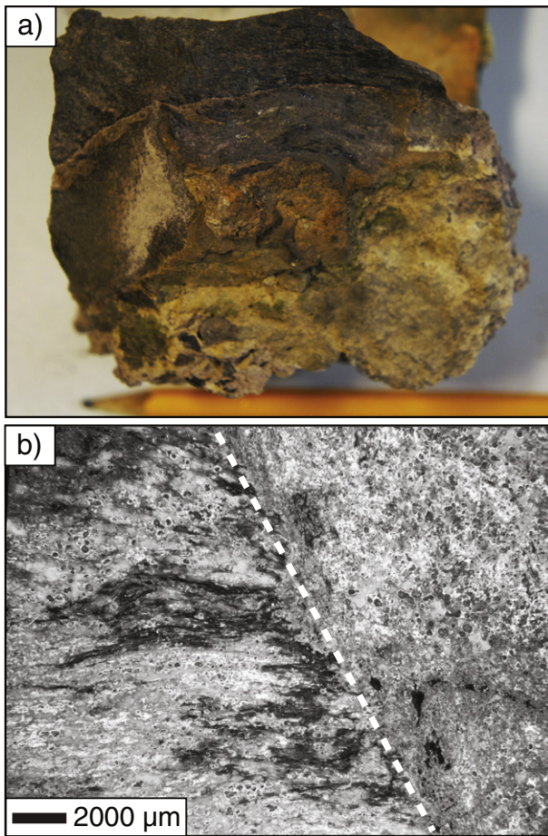
Fig. 8. a) Photograph of breccia sample 47 consisting of broken clasts in a fine-grained matrix. b) Optical microscope image of breccia sample 47 showing a foliation of very high aspect ratio vesicles truncated by a healed fault (dashed white line).
