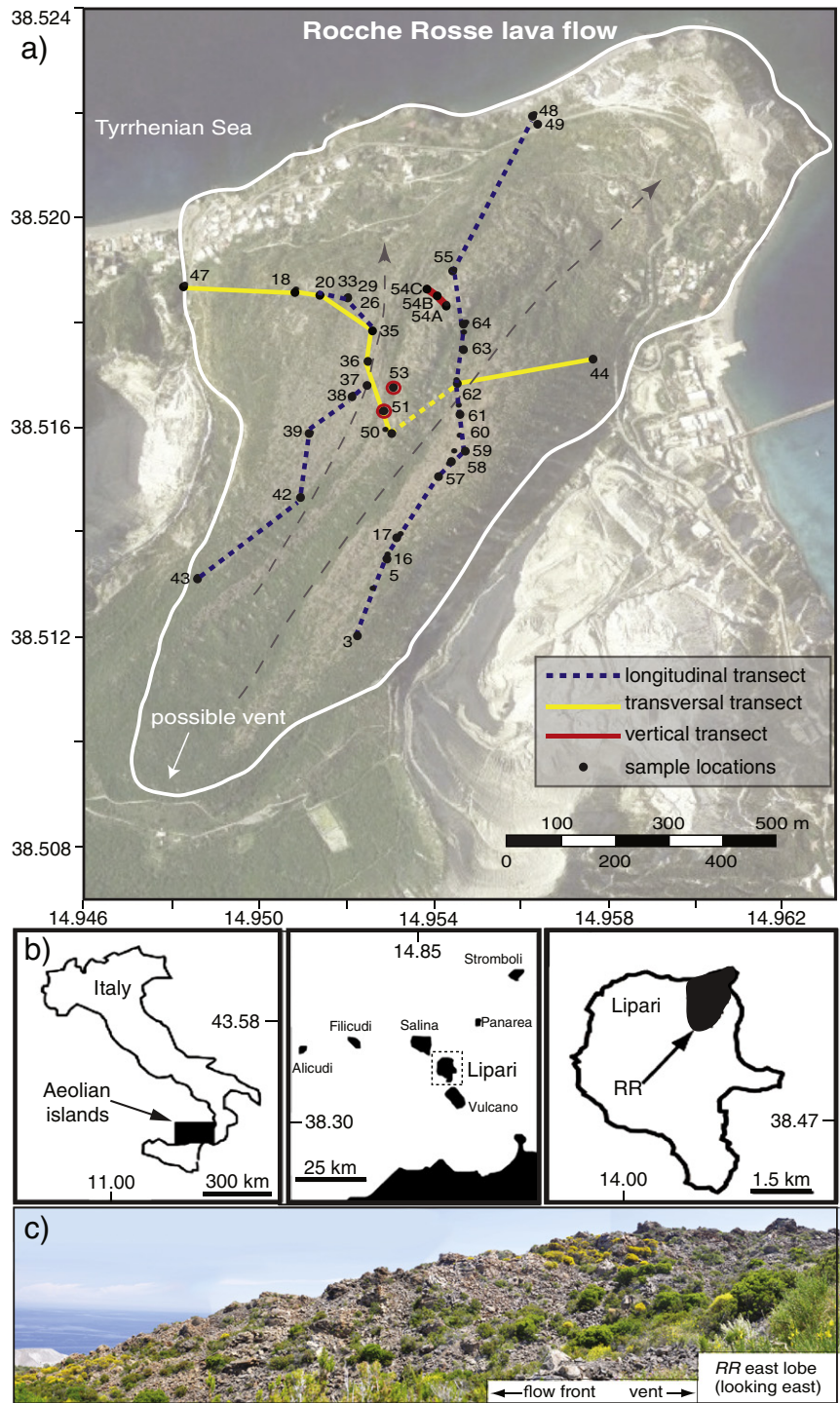
Fig. 1. a) Map of the Rocche Rosse lava flow (source: Google Earth) showing sampling and transect locations. Numbers refer to sample names. Vertical transects (red lines) include multiple samples at each point. Axes are latitudinal and longitudinal coordinates. Flow outline taken from the geological map of Lipari island by (Pichler, n.d.). b) Schematic map of location of Aeolian islands, Lipari and the RR flow, adapted from (Cabrera et al., n.d.). c) Photograph of east lobe of the RR lava flow (credit: L. Caricchi) showing clinkery surface texture and flow ramp features.
