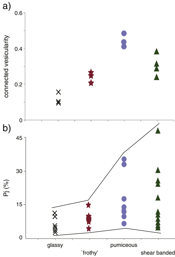
Fig. 7. a) Connected vesicularity of RR lavas analysed by helium pycnometry and b) P_j of all samples measured for AMS, with lines marking upper and lower P_j limits. Symbols represent the respective sample types.
